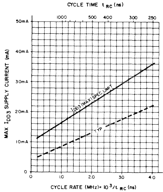
Fig. 3 Maximum I_{DD3} versus cycle rate for device operation at extended frequencies. I_{DD3} (max) curve is defined by the equation: I_{DD3} (max) [mA] = 10 + 6.5 \times cycle rate [MHz].
