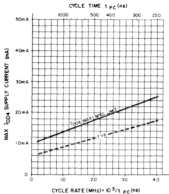
Fig. 4 Maximum I_{DD4} versus cycle rate for device operation in page mode. I_{DD4} (max) curve is defined by the equation: I_{DD4} (max) [mA] = 10 + 3.75 \times cycle rate [MHz].
