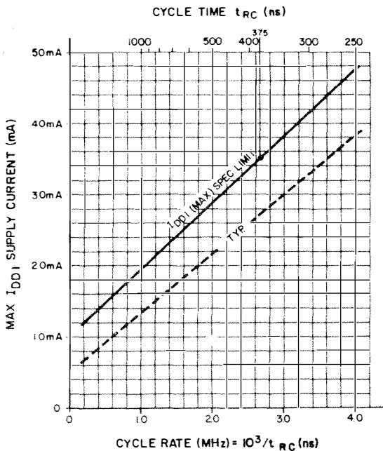
Fig. 2 Maximum I_{DD1} versus cycle rate for device operation at extended frequencies. I_{DD1} (max) curve is defined by the equation: I_{DD1} (max) [mA] = 10 + 9.4 \times cycle rate [MHz].
